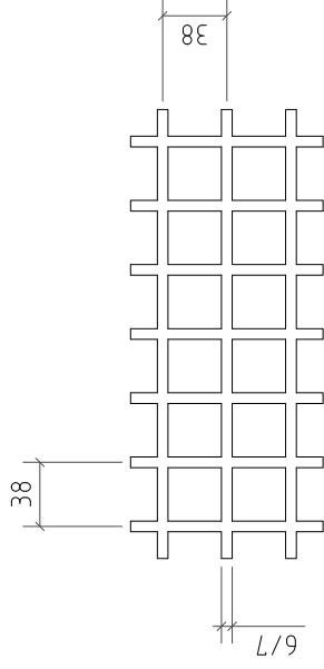
Plan view
