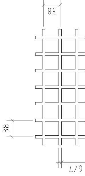
Plan view
